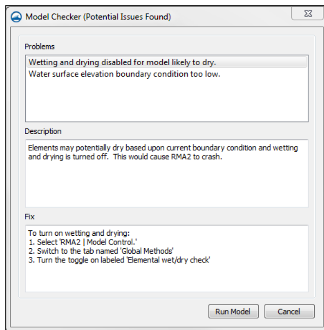
Figure 4 Warning in the Model Checker dialog
