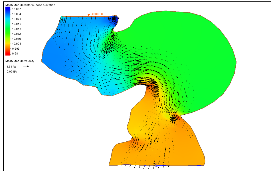
Figure 3 The velocity magnitude solution set
