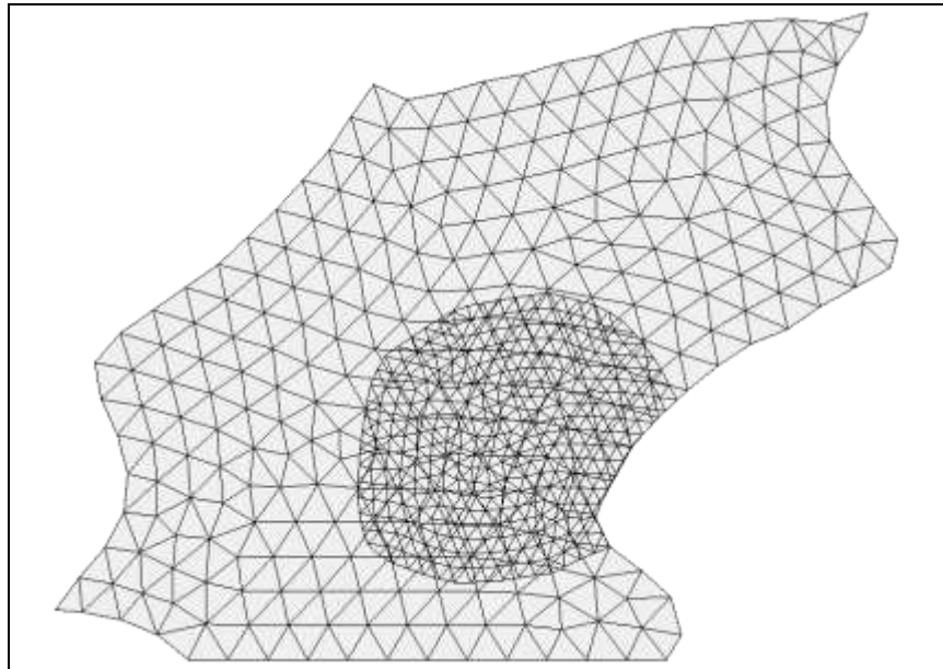
Figure 6 UGrids with overlapping cells
